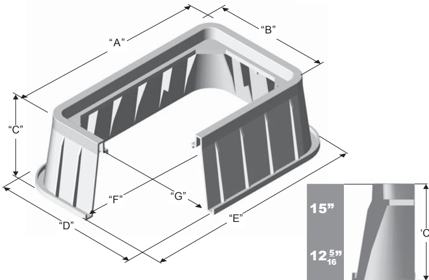
Bolt Down Loc-Kit™ (Patent Pending)
